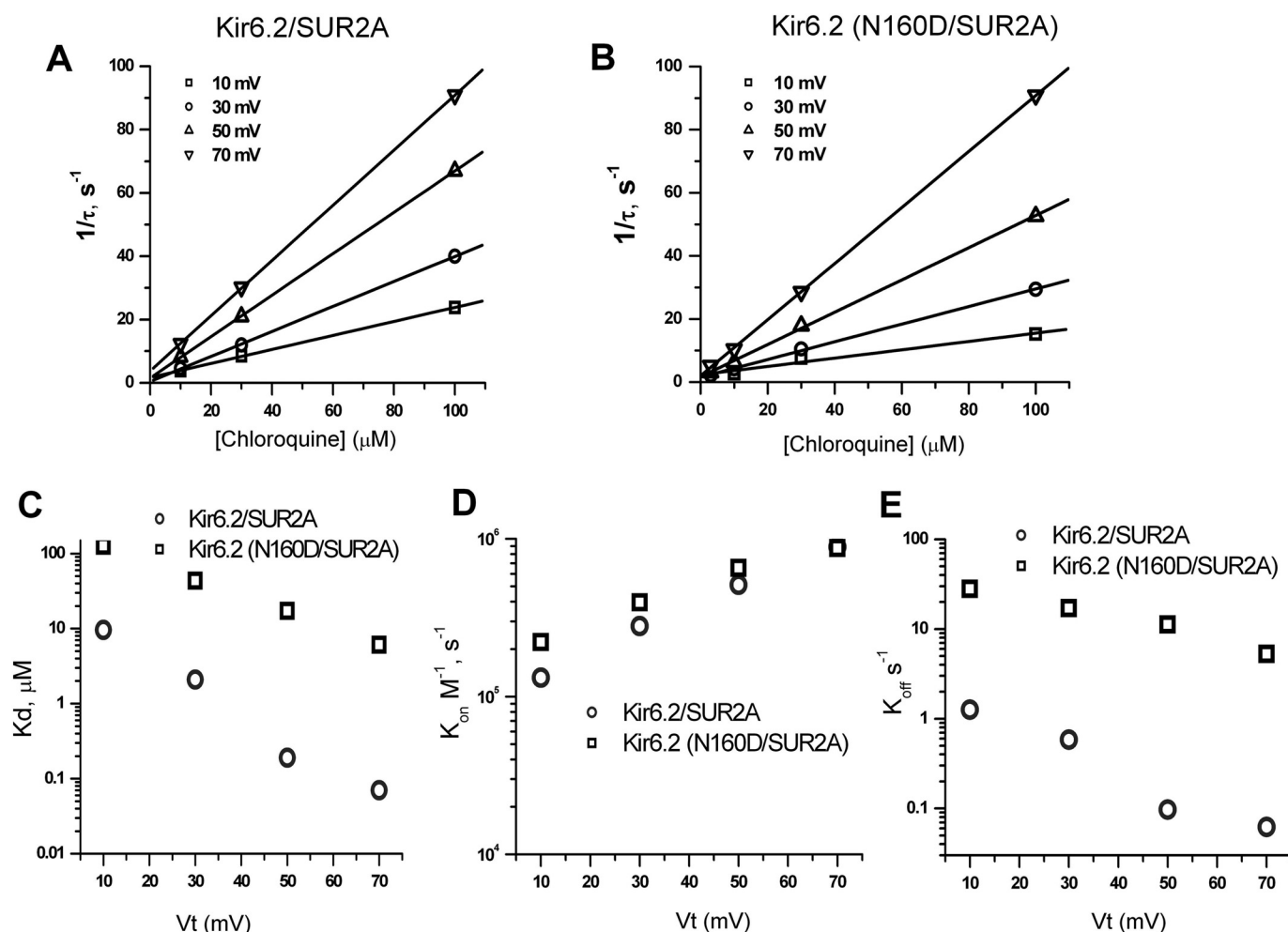
Fig. 6. Kinetic analysis of Kir6.2/SUR2A and Kir6.2 (N160D)/SUR2A blockade by chloroquine. A and B, reciprocals of the time constants ( 1/\tau ) obtained from exponential fits of chloroquine-dependent current relaxation (Figs. 4A and 5A) are plotted against chloroquine concentration at various voltages. Solid lines are linear fits to data. C, K_d values obtained from concentration-dependent inhibition of steady-state currents at different membrane potentials. D, voltage dependence of blocking rate constants ( k_{on} ). E, voltage dependence of the unblocking rate constant ( k_{off} ). Data points were obtained by multiplying K_d by k_{on} for each voltage.
