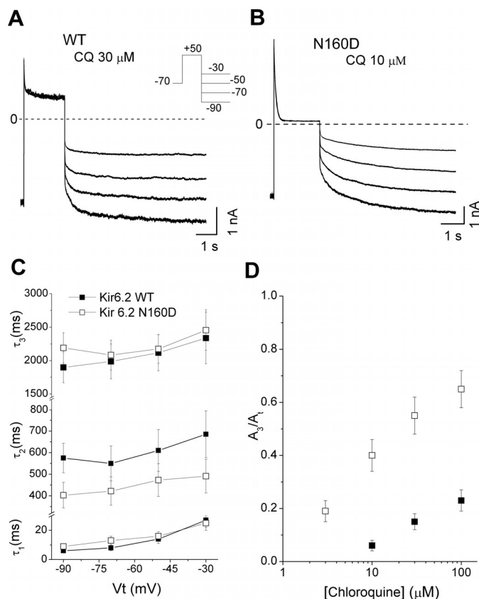
Fig. 7. Chloroquine (CQ) unblock of Kir6.2/SUR2A and Kir6.2(N160D)/SUR2A channels. A and B, current traces from Kir6.2 and Kir6.2(N160D)-containing channels were elicited by a depolarizing voltage step to +50 mV and then repolarizing the membrane to different voltages. C, unblocking time constants were fit with a sum of three exponentials, with time constants plotted as a function of hyperpolarizing test voltage. D, relative amplitude of the component 3 ( A_3/A_1 ) as a function of chloroquine concentration.
